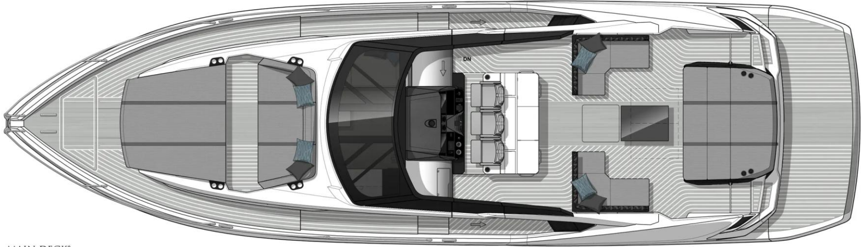
MAIN DECK* Shown with optional side decking
